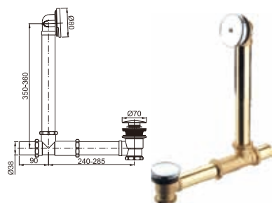
T-shape pop up bath tub drain brass plug
