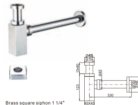
Brass square siphon 1 1/4"
