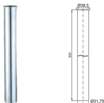
Brass ripple tube Ø31.75
