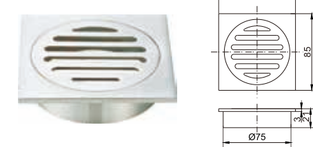
Brass floor drain 4"x4"
