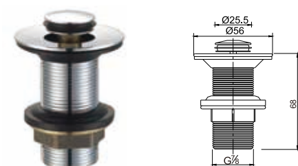
Brass waste for wash basin 7/8" clic-clac
