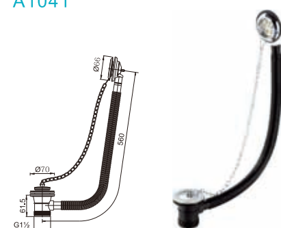
Brass bath tub drain with overflow pipe brass plug with chain
