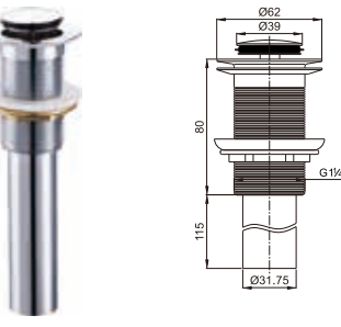
Brass waste for wash basin 1 1/4" clic-clac
