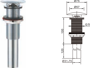
Brass waste for wash basin 1 1/4"
