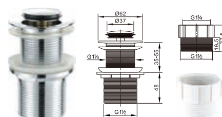
11/4" Brass waste for wash basin with 11/4"-11/2" adapter
