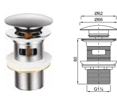
CP Brass & Plastic Pop up
