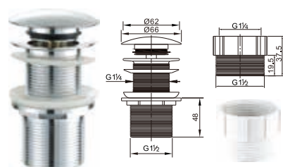
11/4" Brass waste for wash basin with 11/4"-11/2" adapter
