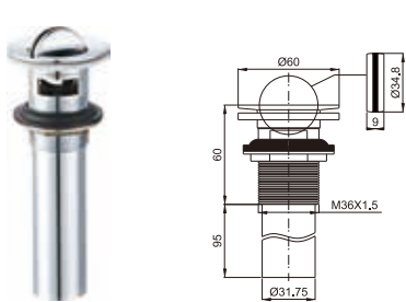
Rotating top waste for washbasin M36x1.5, with overflow
