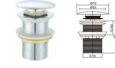
Brass waste for wash basin 1 1/2" clic-clac
