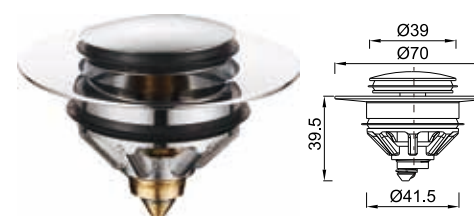
Sink filter plug
