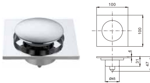
Brass floor drain 4"x4"
