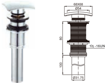
Brass waste for wash basin 1 1/2-16UN clic-clac
