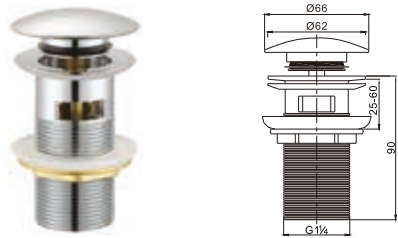
Brass waste for wash basin 1 1/4" with overflow clic-clac
