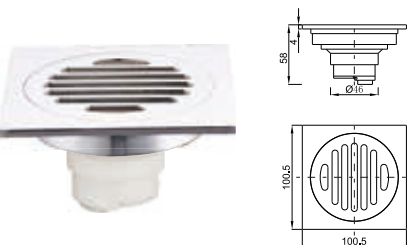
Brass floor drain
