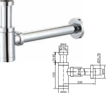
Brass round siphon 1 1/4"
