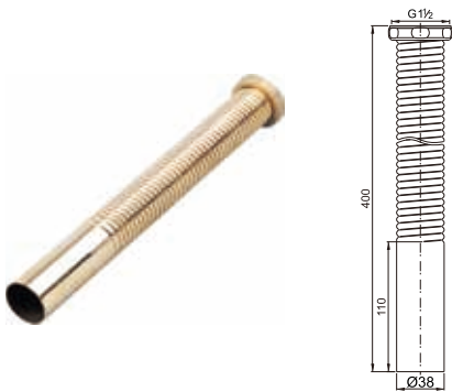
Brass ripple tube for bathtub
