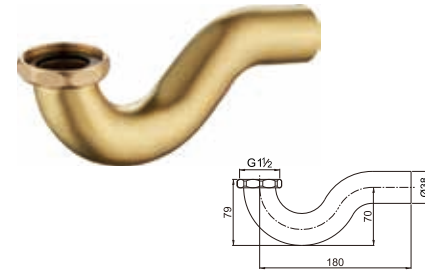
Brass P-tube for bathtub
