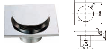
Brass floor drain 4"x4"
