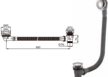
Plastic bath tub drain clic-clac
