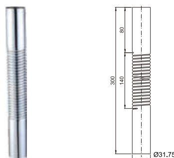
Brass ripple tube Ø31.75
