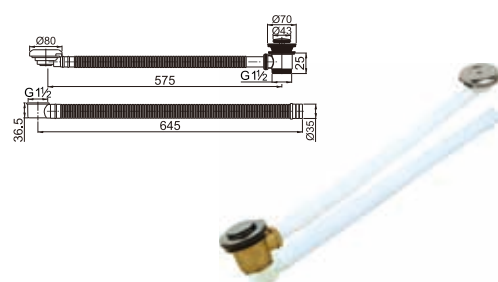
Brass bath tub drain with overflow pipe clic-clac
