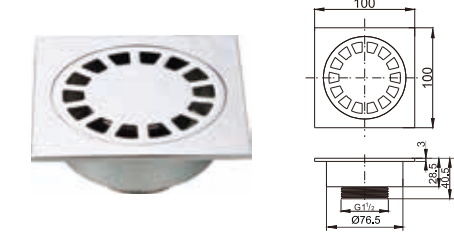
Brass floor drain 4"x4"
