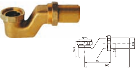
Brass P-tube for bathtub
