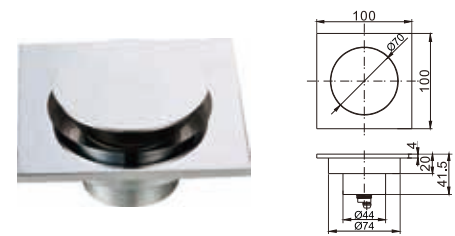
Brass floor drain 4"x4"
