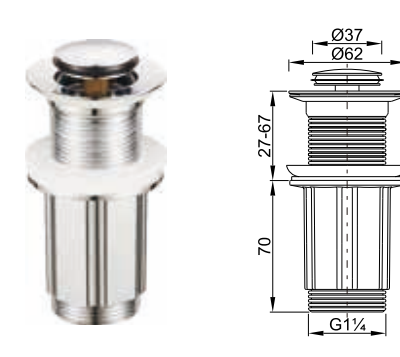
CP Brass & Plastic Pop up
