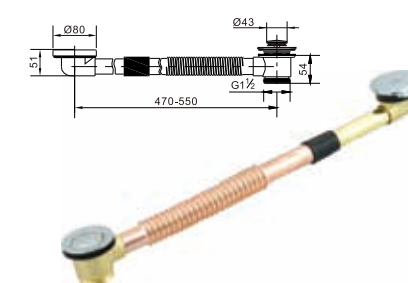
Brass bath tub drain clic-clac
