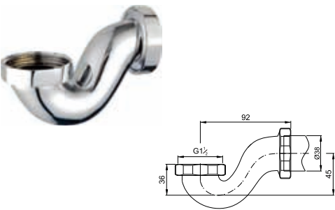
Brass P-tube for bathtub
