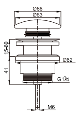
Brass waste for wash basin 1 1/4" clic-clac
