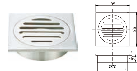
Brass floor drain 4"x4"
