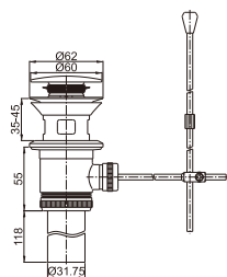
Brass pop-up waste for wash basin 1 1/4"with overflow
