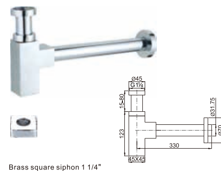
Brass square siphon 1 1/4"
