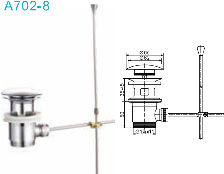
Brass pop-up waste or wash basin 11/4"with overflow
