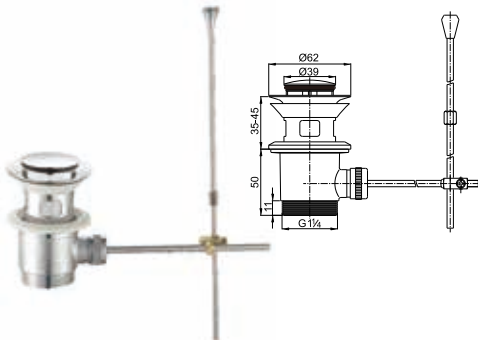
Brass pop-up waste for wash basin 11/4"with overflow
