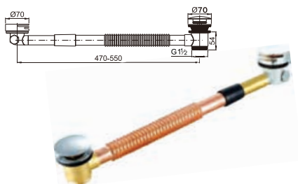
Brass bath tub drain clic-clac
