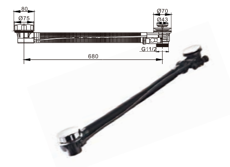
Plastic bath tub drain handle-controlled
