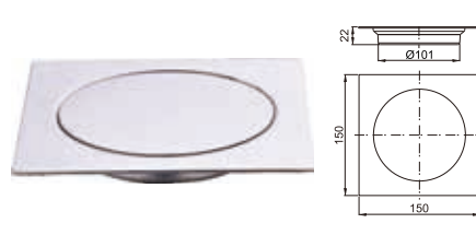
Stainless steel floor drain6"X6"
