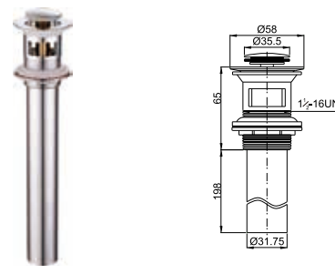
Brass waste for wash basin 1 1/2-16UN with overflow clic-clac
