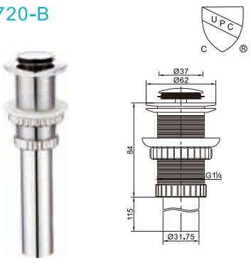
Brass waste for wash basin 1 1/4" clic-clac
