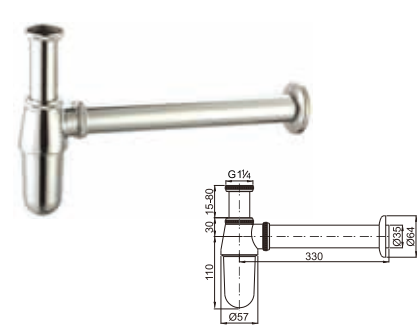
Wall pipe: \phi 35mm
