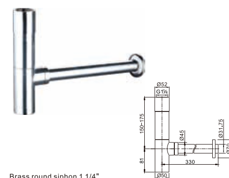
Brass round siphon 1 1/4"
