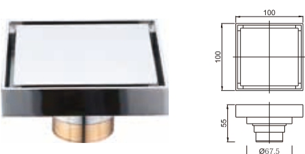
Brass floor drain
