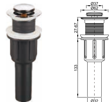
CP Brass & Grey Plastic Pop up
