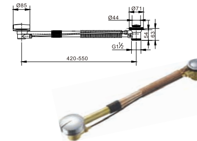
Brass bath tub drain handle-controlled
