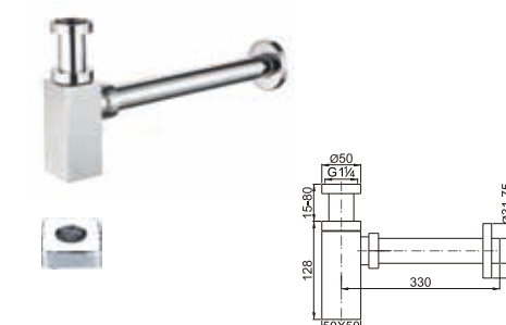
Brass square siphon 1 1/4"
