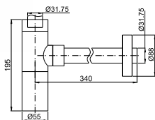
Brass round siphon 1 1/4"
