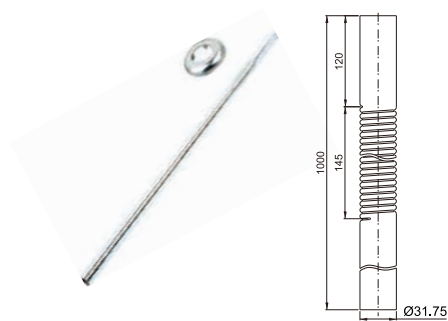
Brass ripple tube Ø31.75
