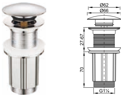
CP Brass & Plastic Pop up
