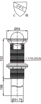
Rotating top waste for washbasin 1 7/16-20UN
