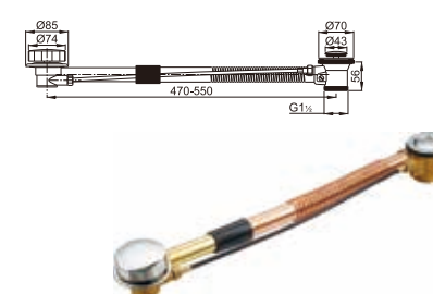
Brass bath tub drain handle-controlled
