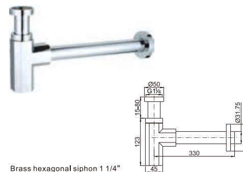
Brass hexagonal siphon 1 1/4"
