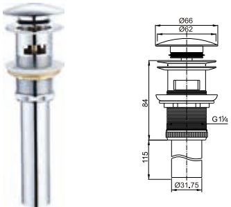
Brass waste for wash basin 1 1/4" clic-clac
