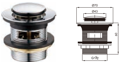
Brass waste for bath 1 1/2", with overflow clic-clac
