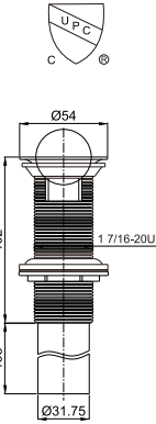
Rotating top waste for washbasin 1 7/16-20UN
