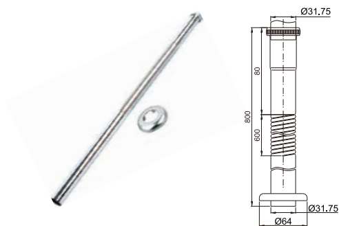
Brass ripple tube Ø31.75
