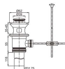
Brass pop-up waste for wash basin 1 1/4"with overflow
