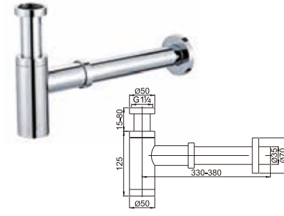
Brass round siphon 1 1/4"
