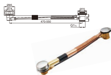
Brass bath tub drain handle-controlled
