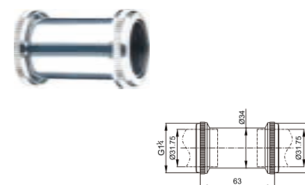
Brass connector with double screw nuts 1 1/4"
