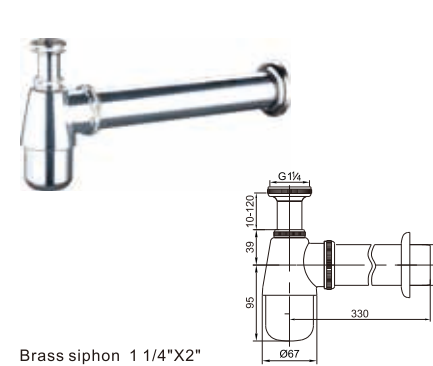
Brass siphon 1 1/4"X2"
