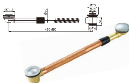
Brass bath tub drain clic-clac
