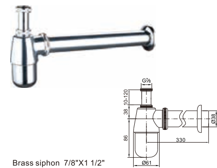
Brass siphon 7/8"X1 1/2"
