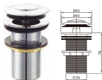
Brass waste for wash basin 1 1/4" without overflow clic-clac
