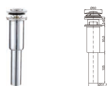
Brass waste for wash basin 1 1/4" clic-clac
