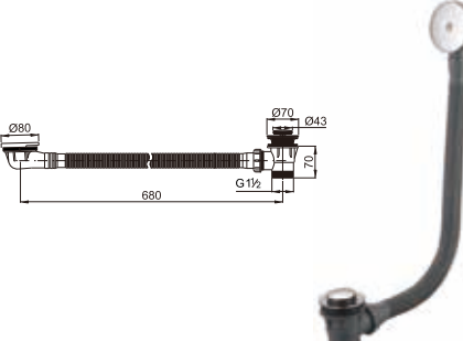
Plastic bath tub drain clic-clac
