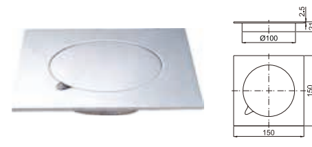
Brass floor drain 6"X6"
