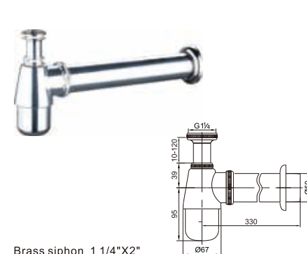
Brass siphon 1 1/4" X 2"
