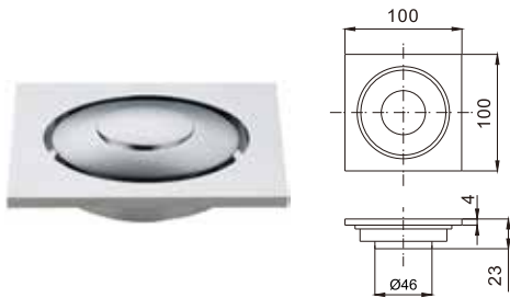
Brass floor drain
