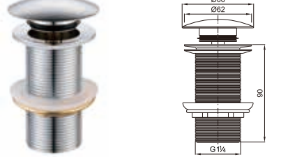
Brass waste for wash basin 1 1/4" clic-clac
