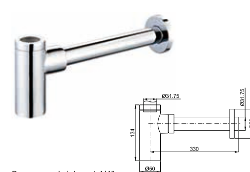
Brass round siphon 1 1/4"
