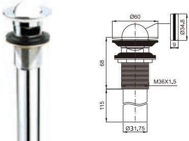
Rotating top waste for washbasin M36x1.5,with overflow
