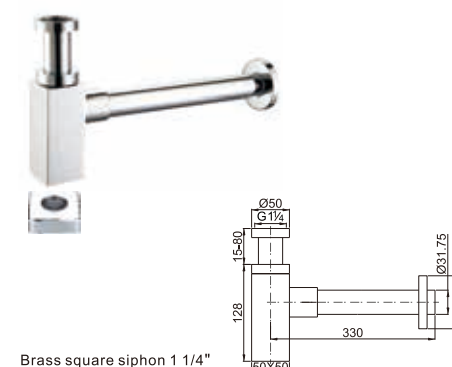
Brass square siphon 1 1/4"
