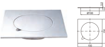
Brass floor drain 6"X6"
