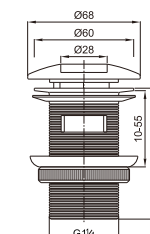
Brass waste for wash basin 1 1/4" with overflow clic-clac
