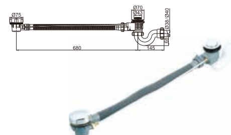
Plastic bath tub drain with p-trap handle-controlled
