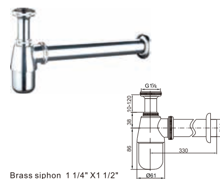
Brass siphon 1 1/4" X1 1/2"
