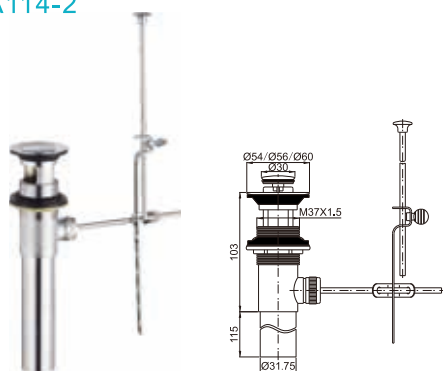
Brass pop-up waste for wash basin M37x1.5with overflow
