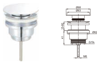
Brass waste for wash basin 1 1/4" clic-clac
