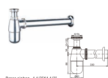
Brass siphon 1 1/2" X 1 1/2"
