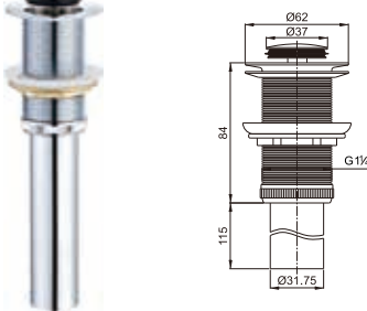
Brass waste for wash basin 1 1/4" clic-clac
