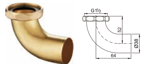
Brass P-tube for bathtub
