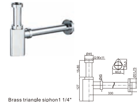
Brass triangle siphon 1 1/4"
