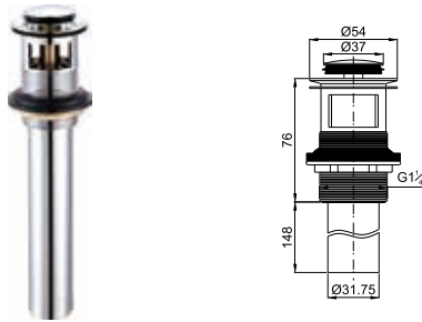
Brass waste for wash basin 1 1/4" with overflow clic-clac
