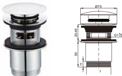
Brass waste for wash basin 1 1/2", with overflow clic-clac
