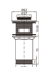
Brass waste for wash basin 1 1/4" with overflow clic-clac
