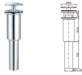
Brass waste for wash basin 1 1/4" fixed cover, not clic-clac
