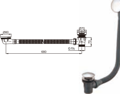
Plastic bath tub drain clic-clac
