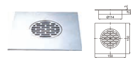
Brass floor drain 6"X6"
