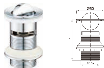
Rotating top waste for wash basin 1 1/4" with overflow
