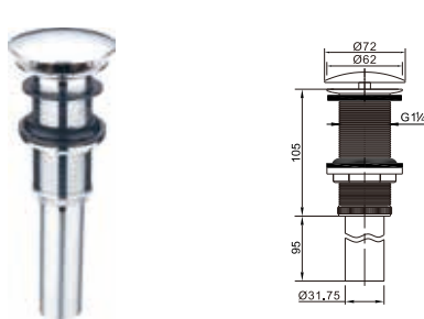
Brass waste for wash basin 1 1/4" fixed cover, not clic-clac
