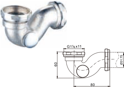
Brass P-tube for bathtub
