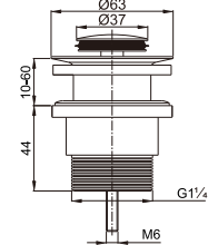
Brass waste for wash basin 1 1/4" clic-clac
