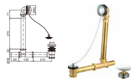
T-shape pop up bath tub drain brass plug
