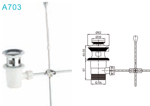
pop-up wastefor wash basin 1 1/4"with overflow
