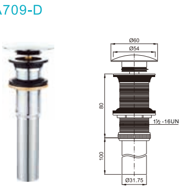
Brass waste for wash basin 1 1/2-16UN clic-clac
