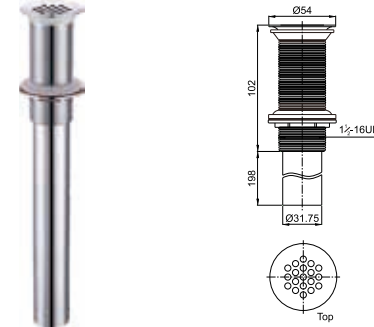
Brass waste for wash basin 1 1/2-16UN fixed cover, not clic-clac
