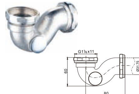
Brass P-tube for bathtub
