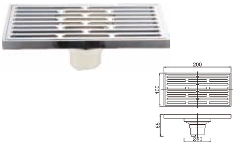
Brass floor drain
