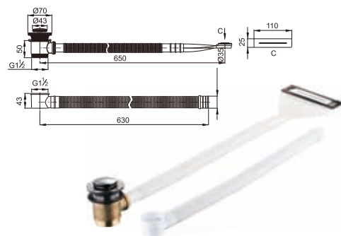
Brass bath tub drain with overflow pipe clic-clac
