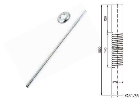
Brass ripple tube Ø31.75
