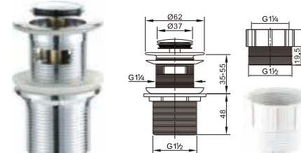
11/4" Brass waste for wash basin with 11/4"-11/2" adapter
