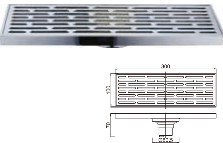
Brass floor drain
