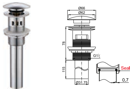
Brass waste for wash basin 1 1/4" clic-clac
