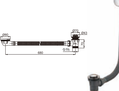
Plastic bath tub drain clic-clac
