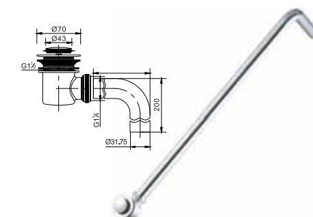
Brass bath drain clic-clac with "L" tube
