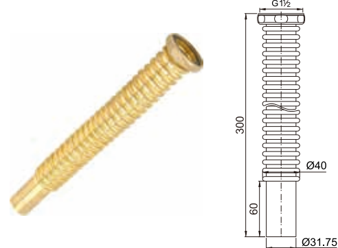
Brass taped tube with screw nut for bathtub
