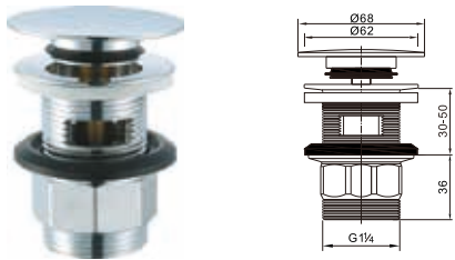
Brass waste for wash basin 1 1/4" with overflow clic-clac
