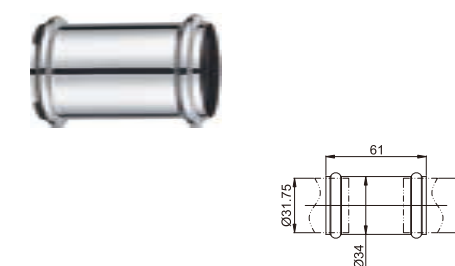
Brass connector with double screw nuts 1 1/4"
