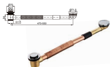
Brass bath tub drain clic-clac
