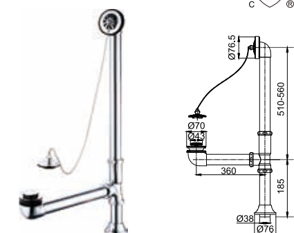
T-shape pop up bath tub drain brass plug
