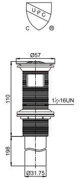
Brass waste for wash basin 1 1/2-16UN with overflow
