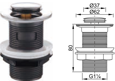
Plastic Pop up with top cover in SUS304
