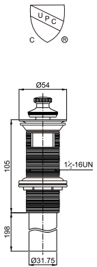
Brass waste for wash basin 1 1/2-16UN
