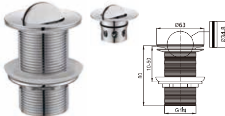
Rotating top waste for washbasin 1 1/4"
