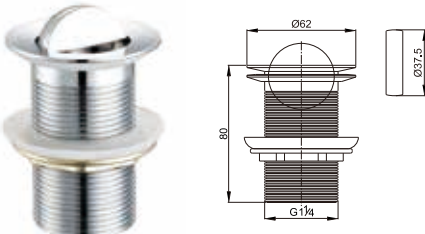
Rotating top waste for washbasin 1 1/4"
