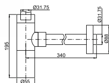
Brass round siphon 1 1/4"
