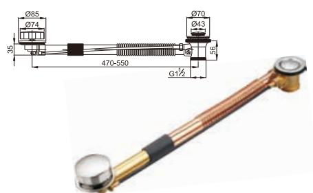
Brass bath tub drain handle-controlled
