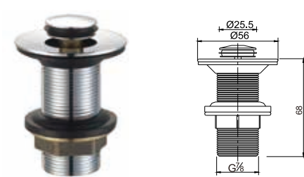
Brass waste for wash basin 7/8"clac-clac
