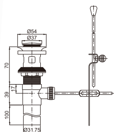
Brass pop-up waste for wash basin 1" with overflow
