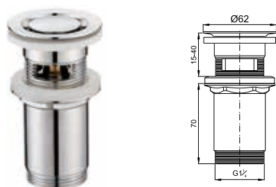
Brass waste for wash basin 1 1/4" clic-clac
