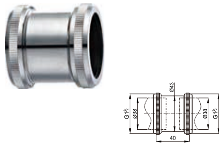
Brass connector with double screw nuts 1 1/2"
