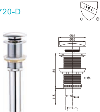
Brass waste for wash basin 1 1/4" clic-clac
