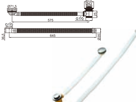
Brass bath tub drain with overflow pipe clic-clac
