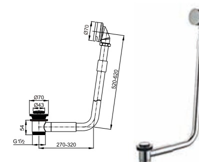
Brass bath tub drain clic-clac
