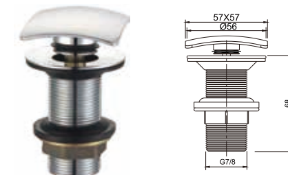
Brass waste for wash basin 7/8" clic-clac
