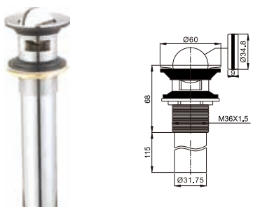
Rotating top waste for washbasin M36x1.5, with overflow
