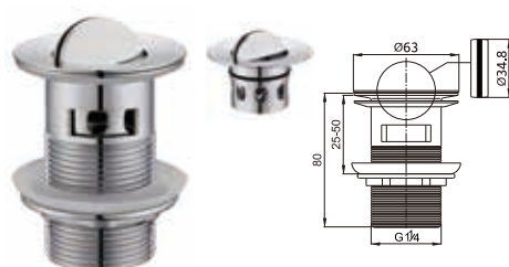
Rotating top waste for wash basin 1 1/4" with overflow
