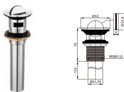
Rotating top waste for washbasin M38x1.5, with overflow
