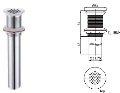
Brass waste for wash basin 1 1/2-16UN fixed cover, not clic-clac
