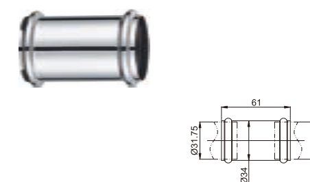
Brass connector with double screw nuts 1 1/4"
