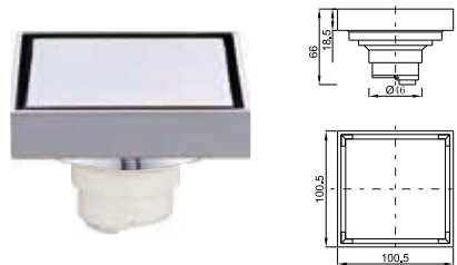
Brass floor drain
