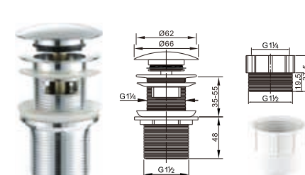
11/4" Brass waste for wash basin with 11/4"-11/2" adapter
