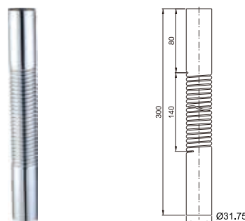
Brass ripple tube Ø31.75
