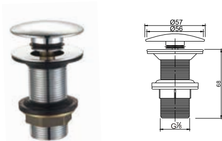
Brass waste for wash basin 7/8"clac-clac
