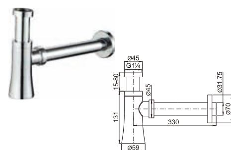
Brass round siphon 1 1/4"
