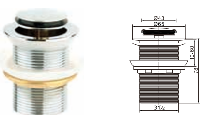
Brass waste for wash basin 1 1/2" clic-clac
