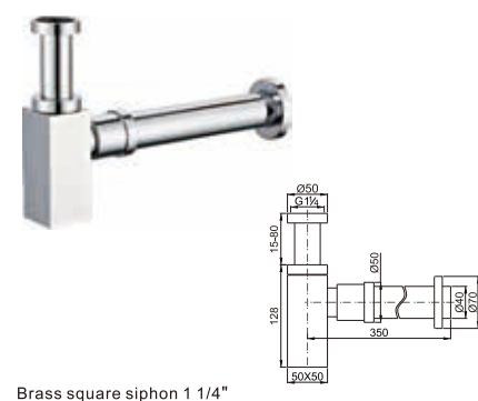
Brass square siphon 1 1/4"
