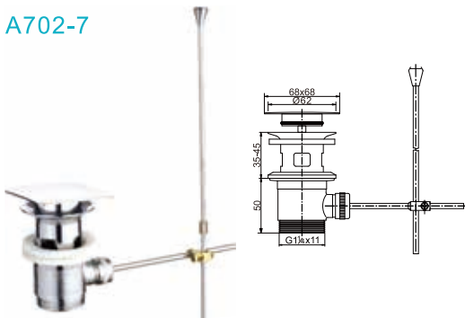
Brass pop-up waste for wash basin 11/4"with overflow
