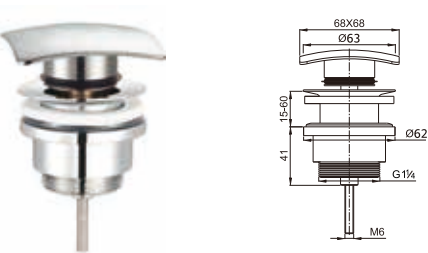
Brass waste for wash basin 1 1/4" clic-clac
