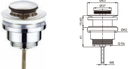
Brass waste for wash basin 1 1/4" clic-clac
