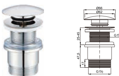
Brass waste for wash basin1 1/2" clic-clac
