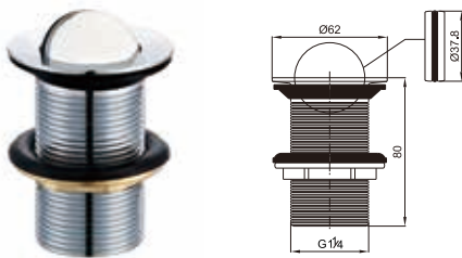
Rotating top waste for washbasin 1 1/4"
