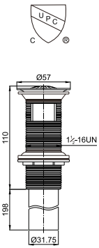
Brass waste for wash basin 1 1/2-16UN with overflow
