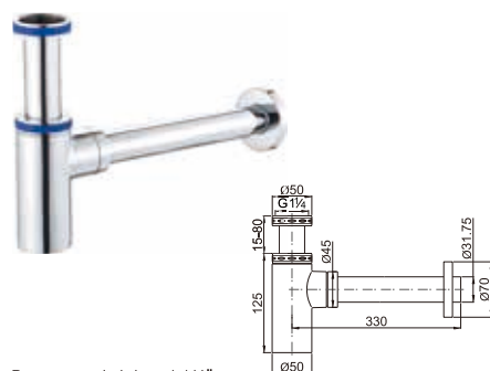
Brass round siphon 1 1/4"
