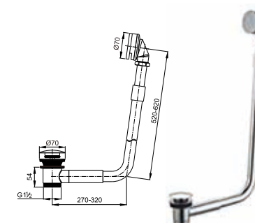
Brass bath tub drain clic-clac
