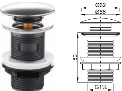
Plastic Pop up with top cover in SUS304
