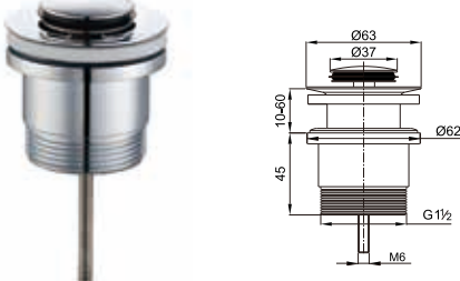
Brass waste for wash basin 1 1/2" clic-clac
