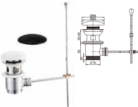
Brass pop-up waste for wash basin 1 1/4"with overflow
