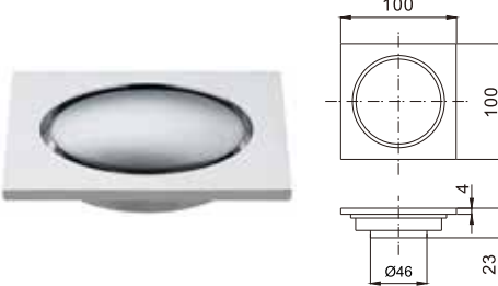
Brass floor drain
