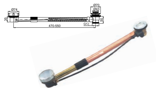
Brass bath tub drain handle-controlled
