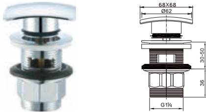
Brass waste for wash basin 1 1/4" with overflow clic-clac
