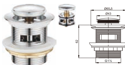
Brass waste for bathtub 1 1/2"
