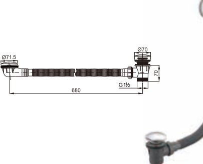
Plastic bath tub drain clic-clac
