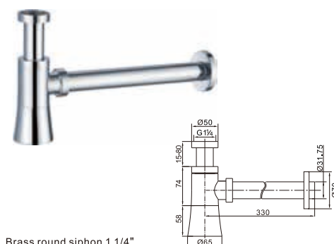
Brass round siphon 1 1/4"
