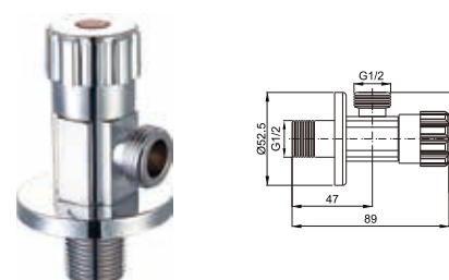
Round angle valve 1/2"
