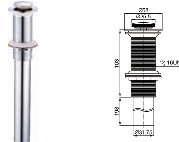
Brass waste for wash basin 1 1/2-16UN clic-clac
