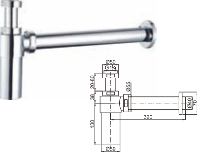
Brass round siphon 1 1/4"
