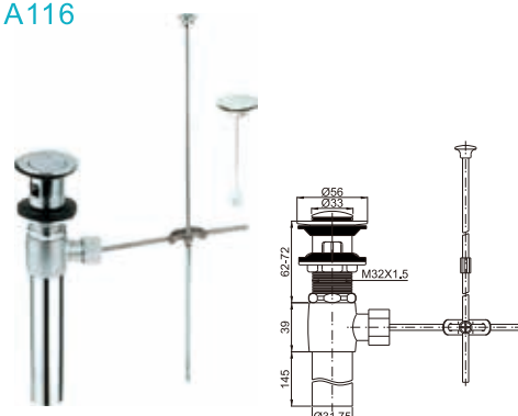
Brass pop-up waste for wash basin M32X1.5with overflow
