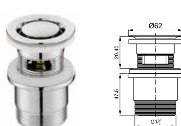
Brass waste for wash basin 1 1/2" clic-clac
