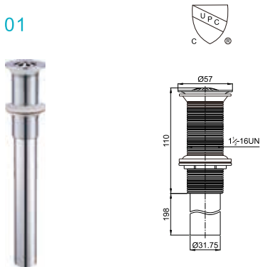
Brass waste for wash basin 1 1/2-16UN fixed cover, not clic-clac
