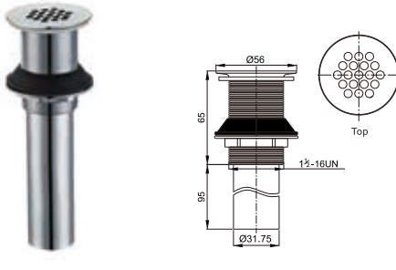
Brass waste for public wash basin 1 1/2-16UN
