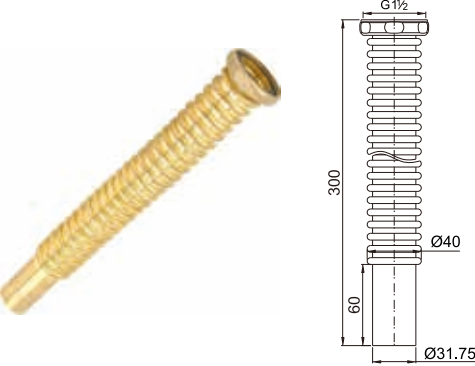
Brass taped tube with screw nut for bathtub
