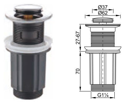
Plastic Pop up with top cover in SUS304
