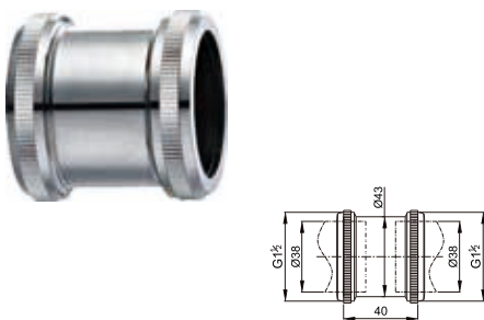
Brass connector with double screw nuts 1 1/2"
