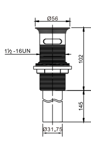
Brass waste for wash basin 1 1/2"x16UN with overflow
