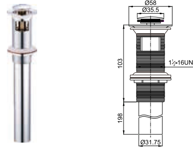
Brass waste for wash basin 1 1/2-16UN with overflow clic-clac
