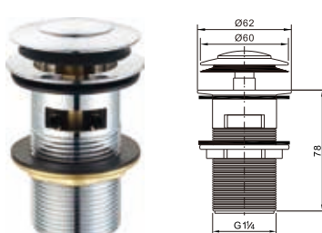
Brass waste for wash basin 1 1/4" with overflow clic-clac
