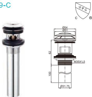
Brass waste for wash basin M35x1.5 clic-clac
