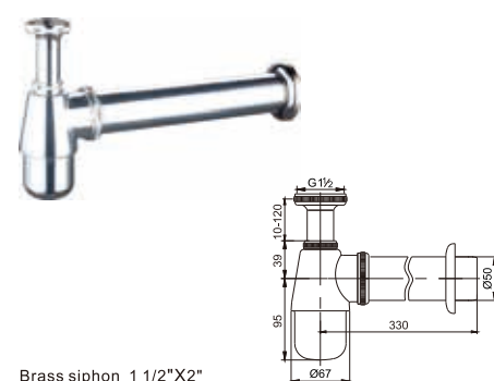
Brass siphon 1 1/2" X 2"
