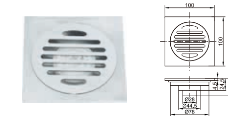
Brass floor drain 4"x4"
