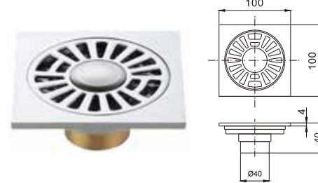
Brass floor drain
