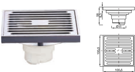
Brass floor drain
