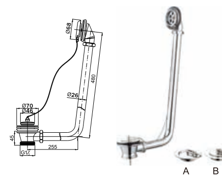
Brass bath tub drain with overflow pipe brass plug with chain
