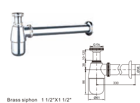
Brass siphon 1 1/2"X1 1/2"
