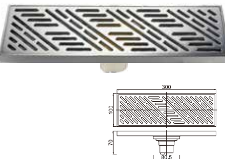
Stainless steel floor drain
