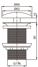
Brass waste for public wash basin 1 1/4" fixed cover not clic-clac
