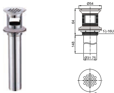
Brass waste for wash basin 1 1/2-16UN with overflow
