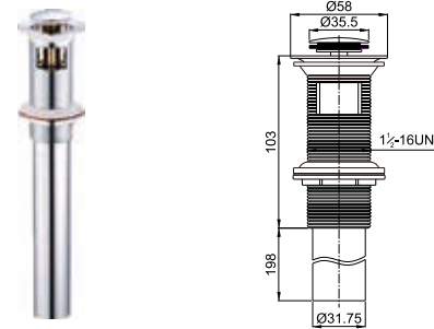
Brass waste for wash basin 1 1/2-16UN with overflow clic-clac
