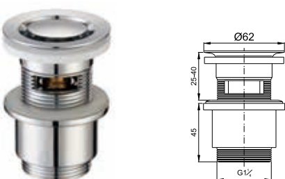
Brass waste for wash basin 1 1/4" clic-clac
