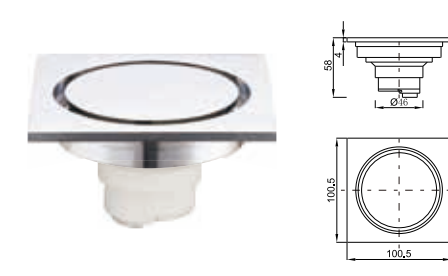
Brass floor drain
