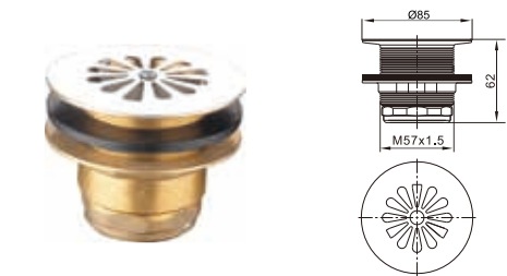
Brass floor drain
