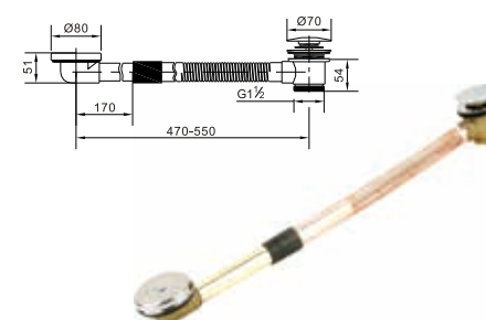
Brass bath tub drain clic-clac
