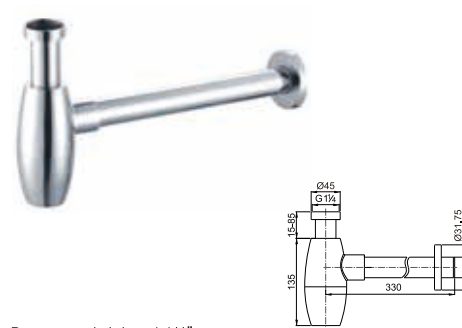
Brass round siphon 1 1/4"
