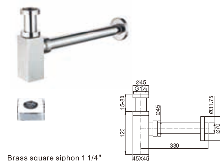
Brass square siphon 1 1/4"
