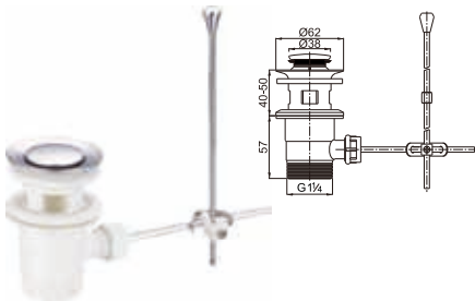
Pop-up wastefor wash basin 1 1/4"with overflow
