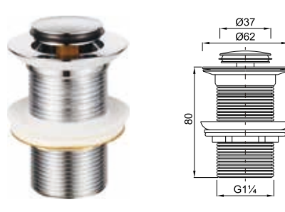
CP Brass & Plastic Pop up
