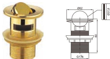
Rotating top waste for wash basin 1 1/4" with overflow
