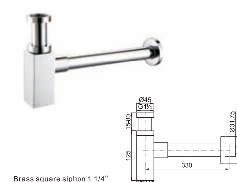
Brass square siphon 1 1/4"
