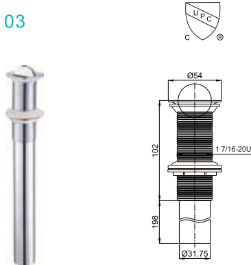
Rotating top waste for washbasin 1 7/16-20UN
