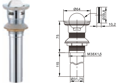
Rotating top waste for washbasin M38x1.5, with overflow
