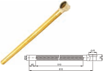
Brass taped tube for bathtub
