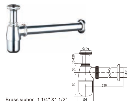
Brass siphon 1 1/4" X 1 1/2"
