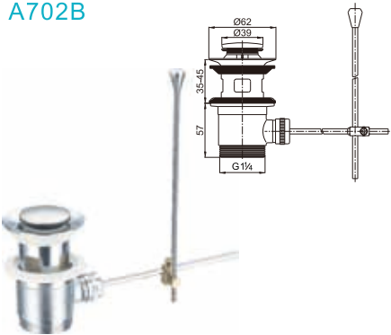
Brass pop-up waste for wash basin 1 1/4"with overflow
