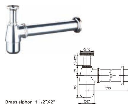
Brass siphon 1 1/2"X2"
