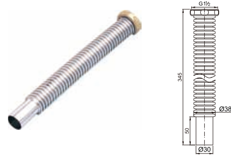
Brass ripple tube for bathtub
