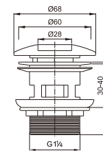
Brass waste for wash basin 1 1/4" clic-clac
