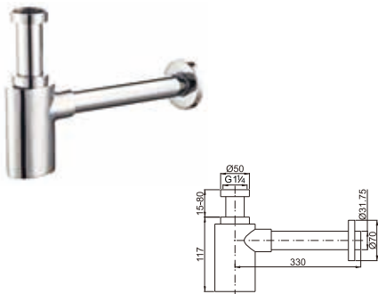
Brass oval siphon 1 1/4"
