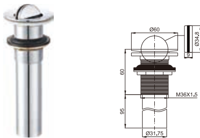
Rotating top waste for washbasin M36x1.5,
