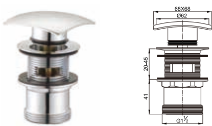
Brass waste for wash basin1 1/2"with overflow clic-clac
