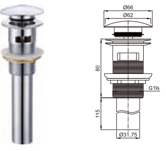
Brass waste for wash basin 1 1/4" clic-clac
