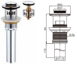
Brass waste for wash basin 1 1/4" clic-clac
