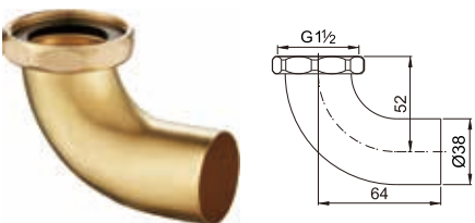
Brass P-tube for bathtub
