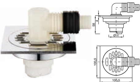
Brass floor drain
