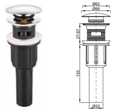
CP Brass & Grey Plastic Pop up
