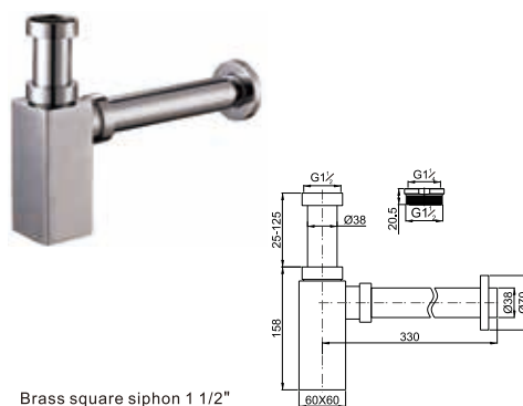
Brass square siphon 1 1/2"
