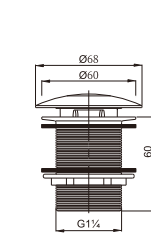
Brass waste for wash basin 1 1/4" clic-clac
