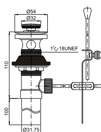
Brass pop-up waste for wash basin 1 5/16X18UNEF with overflow
