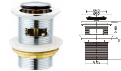
Brass waste for wash basin 1 1/2" with overflow clic-clac
