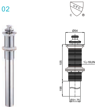
Brass waste for wash basin 1 1/2-16UN
