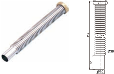
Brass ripple tube for bathtub
