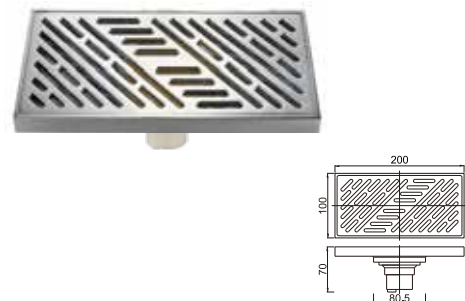
Brass floor drain
