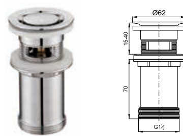
Brass waste for wash basin 1 1/2" clic-clac
