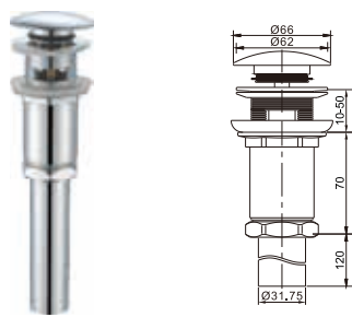
Brass waste for wash basin 1 1/4" clic-clac
