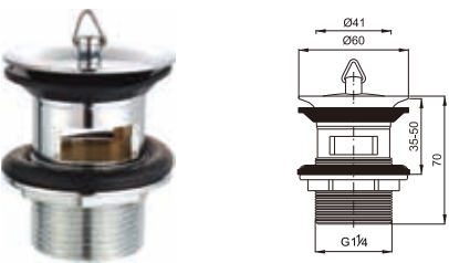
Brass waste for wash basin 1 1/4", with overflow brass plug
