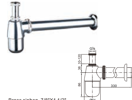
Brass siphon 7/8" X 1 1/2"
