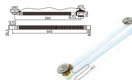
Brass bath tub drain with overflow pipe rubber plug with chain
