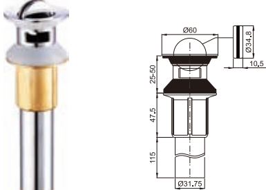
Rotating top waste for washbasin
