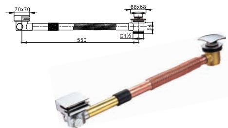
Brass bath tub drain clic-clac
