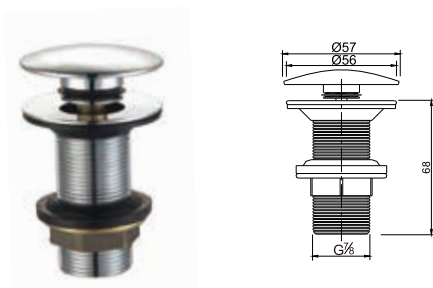
Brass waste for wash basin 7/8" clic-clac
