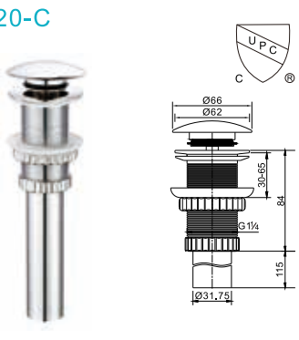
Brass waste for wash basin 1 1/4" clic-clac
