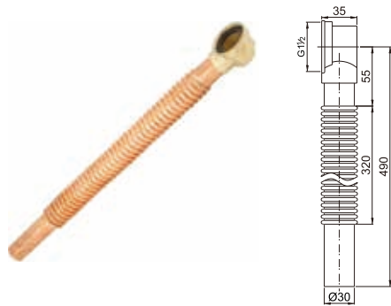
Brass ripple tube for bathtub
