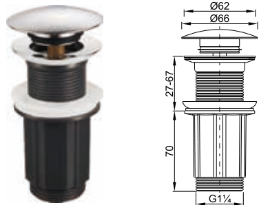
CP Brass & Grey Plastic Pop up
