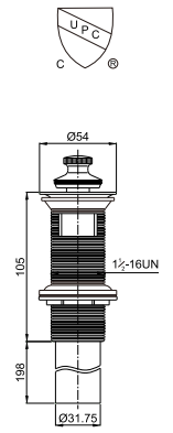
Brass waste for wash basin 1 1/2-16UN
