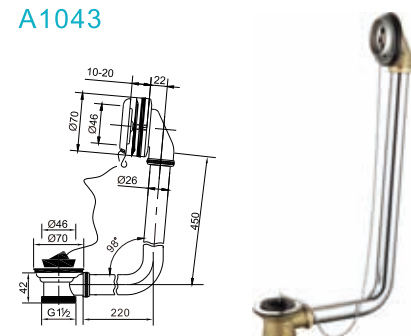
Brass bath tub drain with overflow pipe rubber plug with chain
