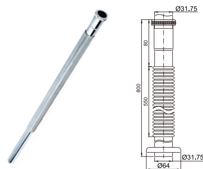
Brass ripple tube Ø31.75
